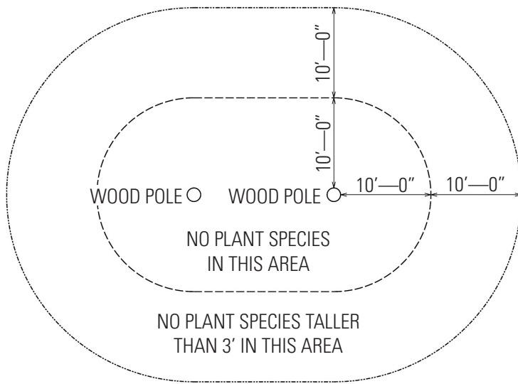
WOOD POLE STRUCTURE THREE POLE STRUCTURE SIMILAR
