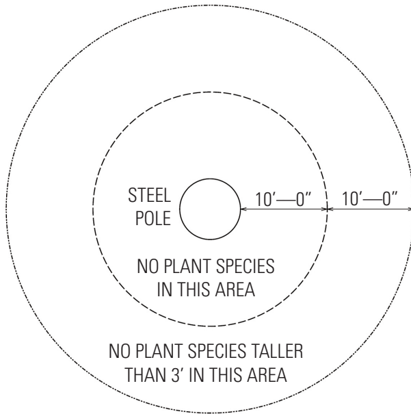
STEEL POLE STRUCTURE
