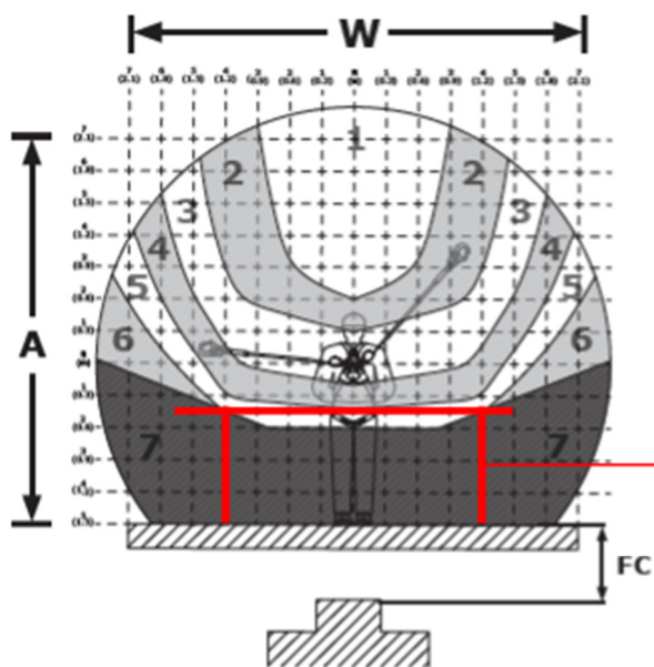
Fall Clearance Chart #3: 311 lb. - 420 lb. (141 kg - 191 kg)
