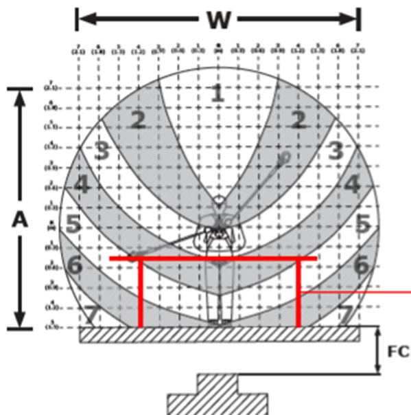
Fall Clearance Chart #1: 130 lb. - 220 lb. (59 kg - 100 kg)
