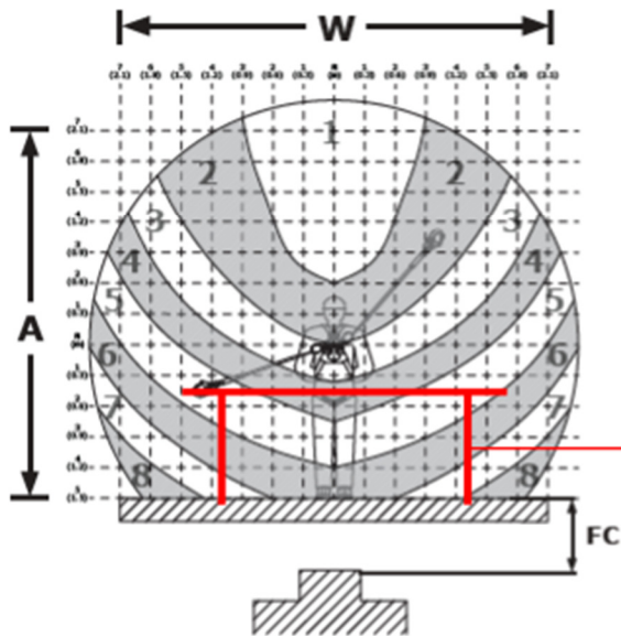
Fall Clearance Chart #2: 221 lb. - 310 lb. (101 kg - 140 kg)
