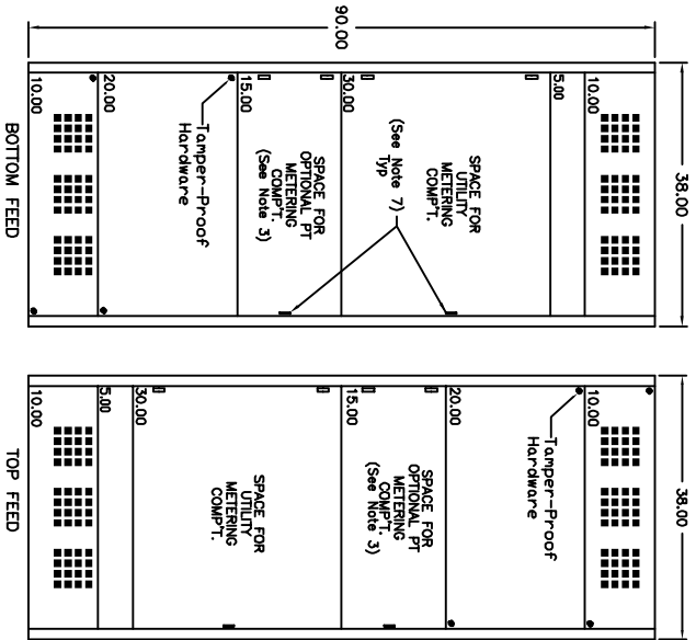
FIG. 5 AMEREN CT COMPARTMENT FRONT ELEVATIONS FOR WINDOW-TYPE CT'S 1201-4000A (480 or 208V)
