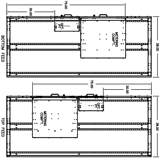
FIG. 6 AMEREN CT COMPARTMENT SIDE VIEWS FOR WINDOW-TYPE CT'S 1201-4000A (480 or 208V) (38D SHOWN)
