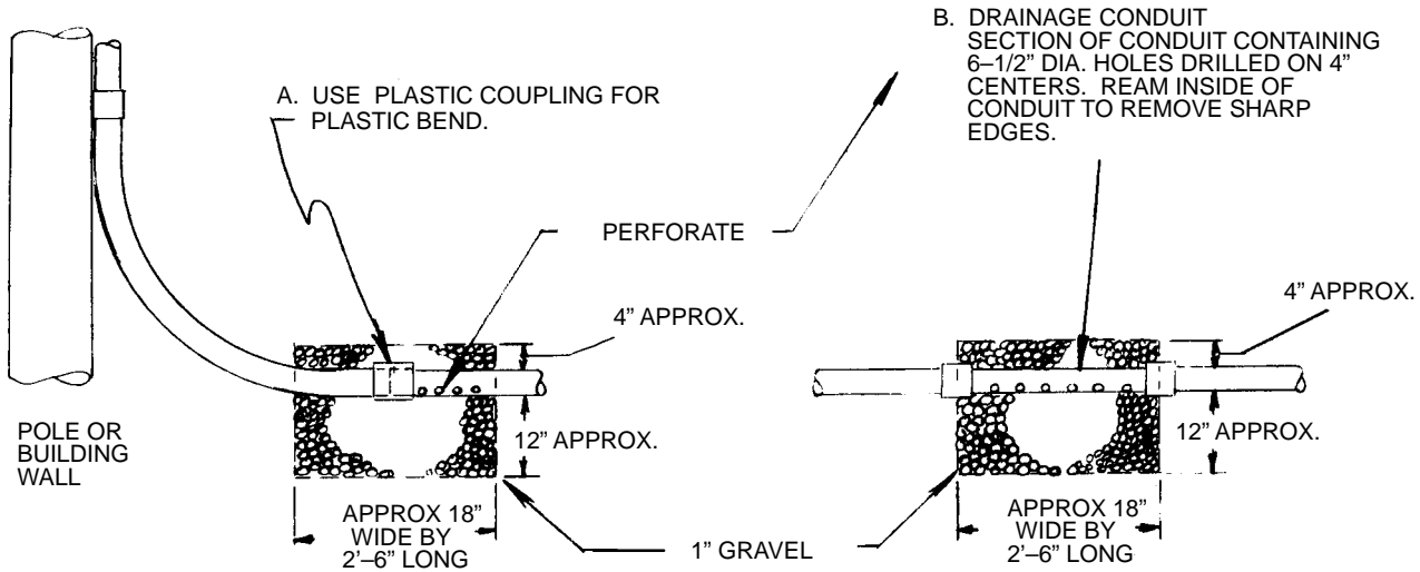
FIG. 1 FOR BURIED ELECTRICAL PLASTIC CONDUIT
