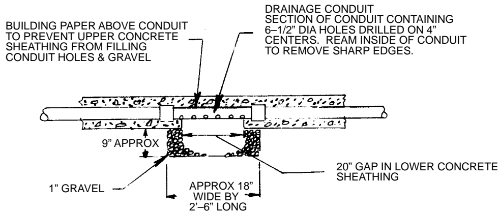
FIG. 3 FOR CONCRETE ENCASED PLASTIC CONDUIT AT LOWEST POINT IN RUN
